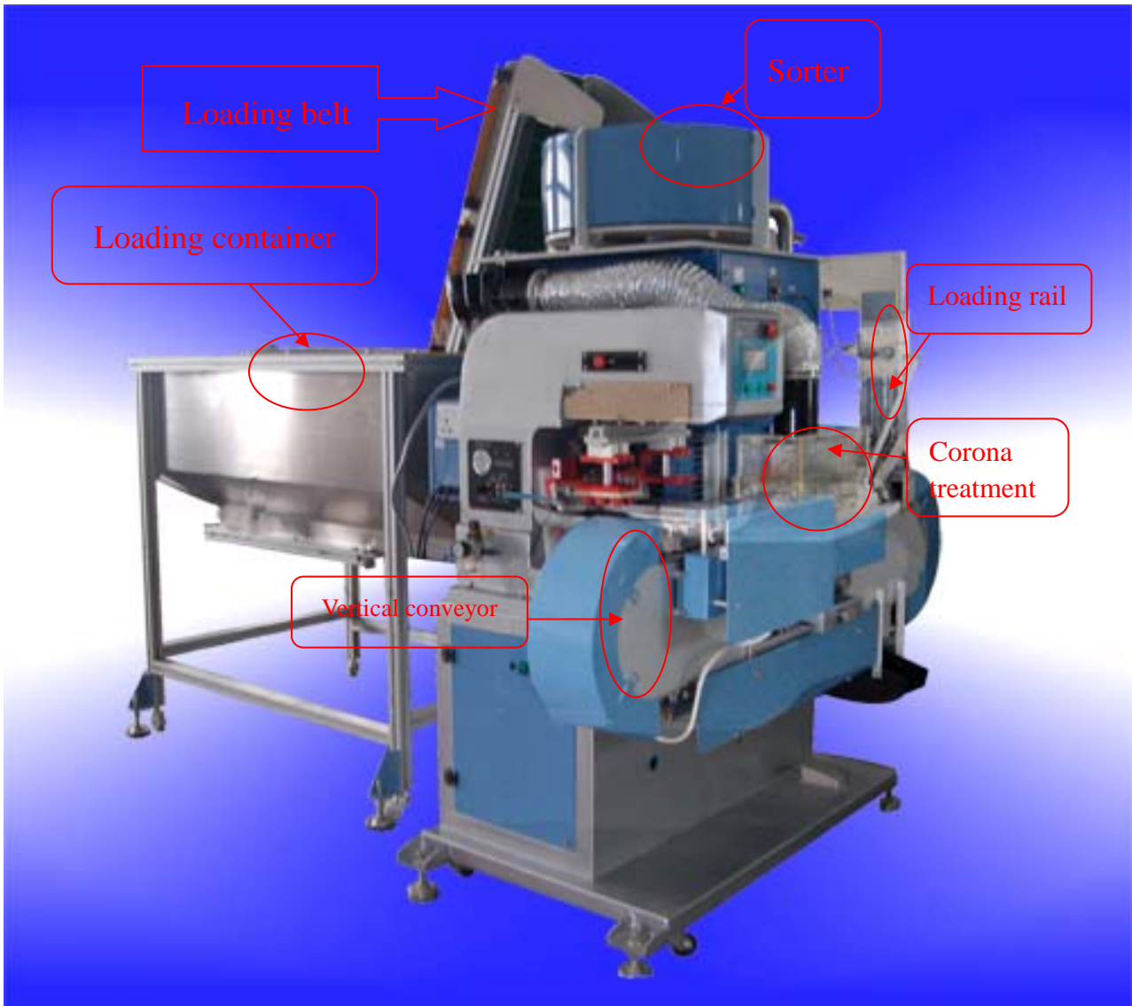
ACP152VCA auto two color pad printer with vertical conveyor (picture showing ink tray type machine)
